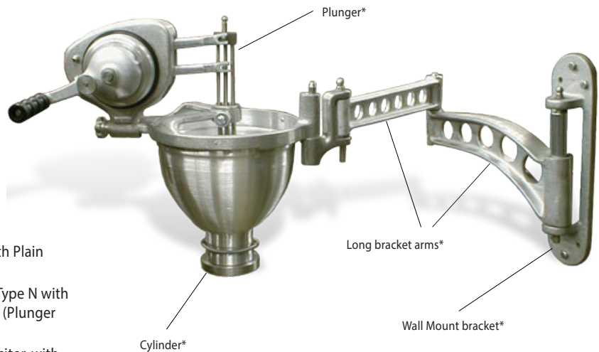
Belshaw Type N shown with wall mount and long extend arms, for bolting to a wall.
