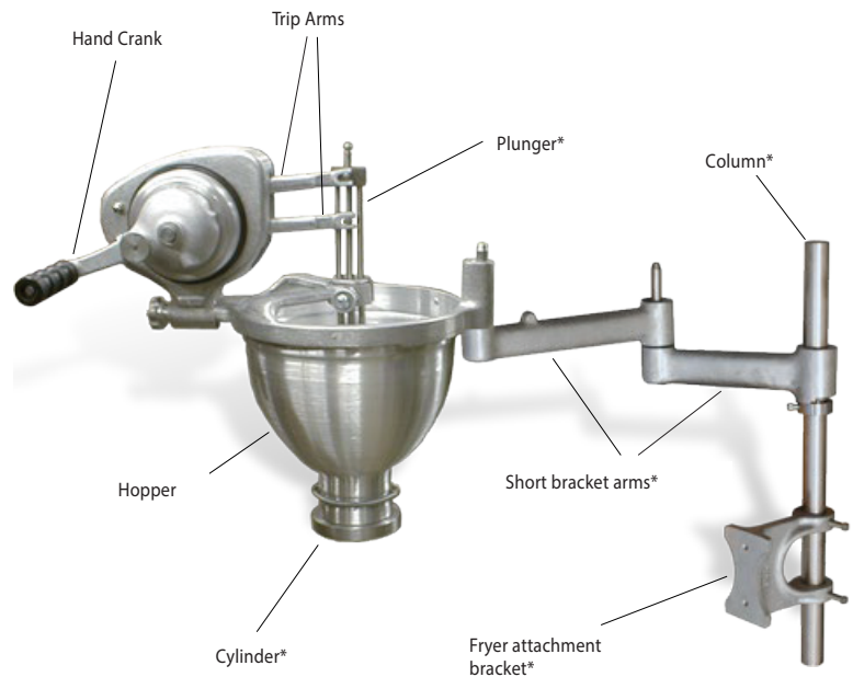
Belshaw Type N shown with column mount and long extend arms, as used for Belshaw Adamatic 'Cut-N-Fry'
